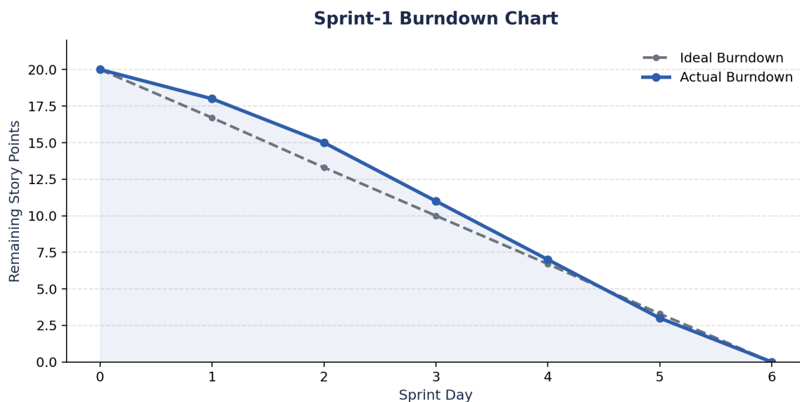
Figure: Sprint-1 ideal vs. actual burndown for the ServiceNow-Based Employee Laptop Request Application.
